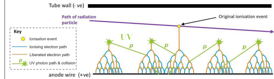
Spread of avalanches in a Geiger-Muller tube
